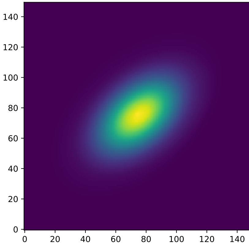
Ellipse Model
